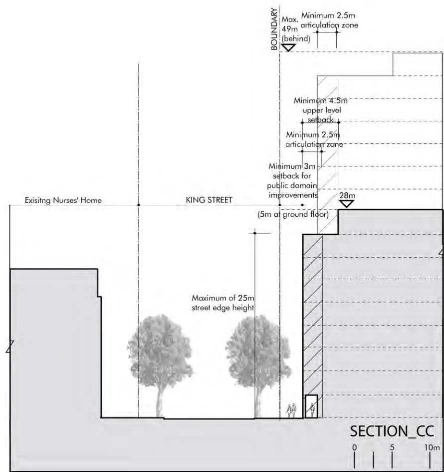
Figure 9: King Street typical street cross-section C-C
